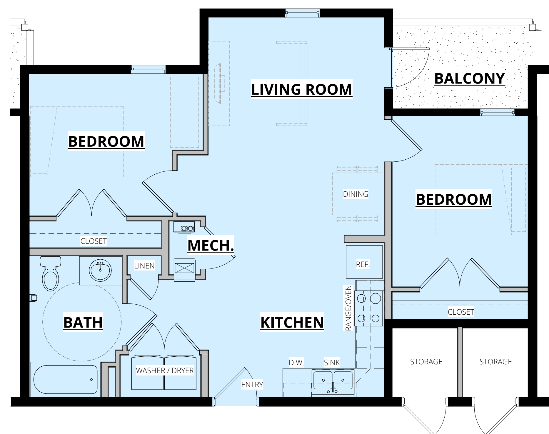
2 ENLARGED FLOOR PLAN 2-BEDROOM UNIT
