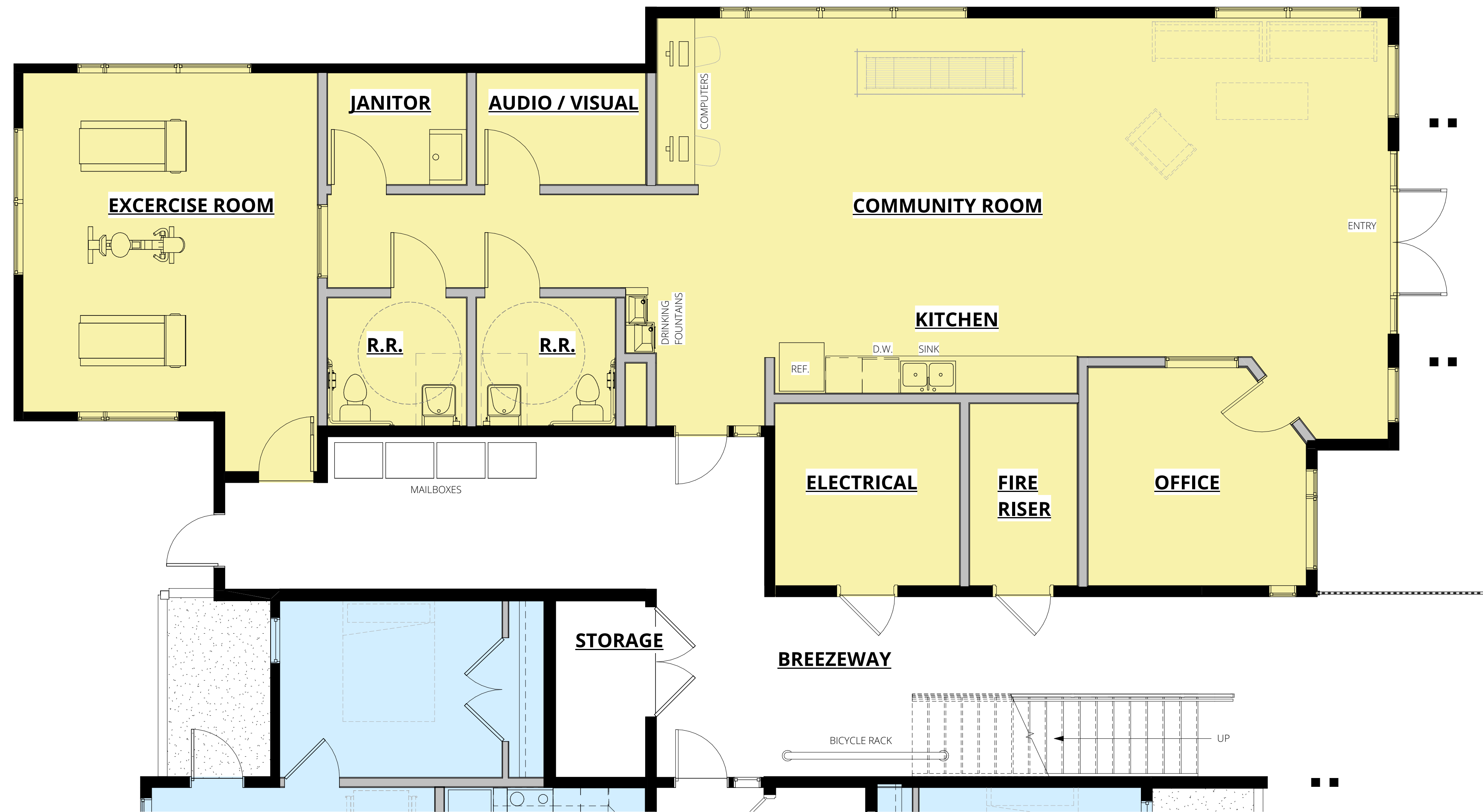
3 ENLARGED FLOOR PLAN COMMUNITY ROOM
