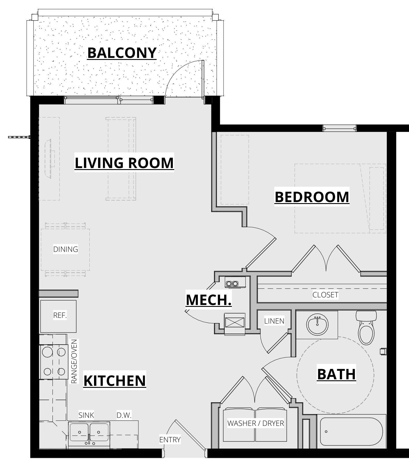
1 ENLARGED FLOOR PLAN 1-BEDROOM UNIT
